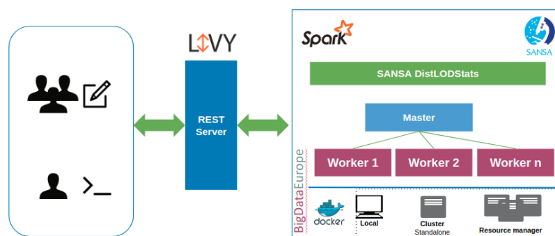
Fig. 1. STATisfy overview architecture.
